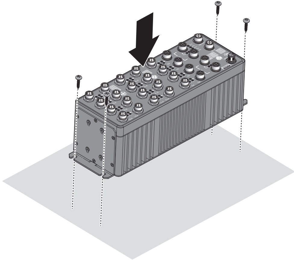
Figure 2.2 Installing a Switch on Flat Surface
