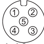
Figure 2.11 M12 A-Coded Connector Pin Assignment
