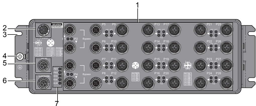
Figure 1.1 Front View
