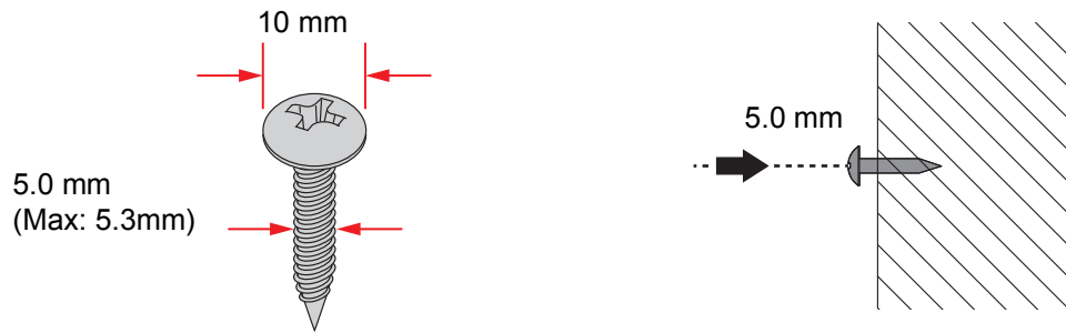
Figure 2.3 Securing Wall Mounting Screws
