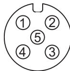
Figure 2.12 Alarm Port Pin Assignment
