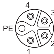
Figure 2.8 ETH Port
