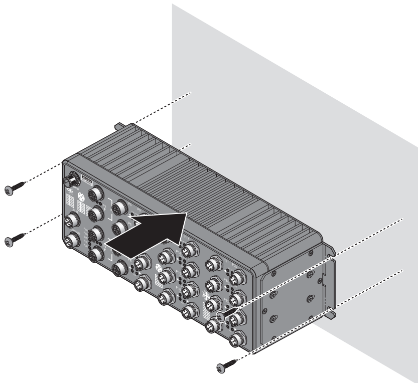
Figure 2.4 Switch Installation
