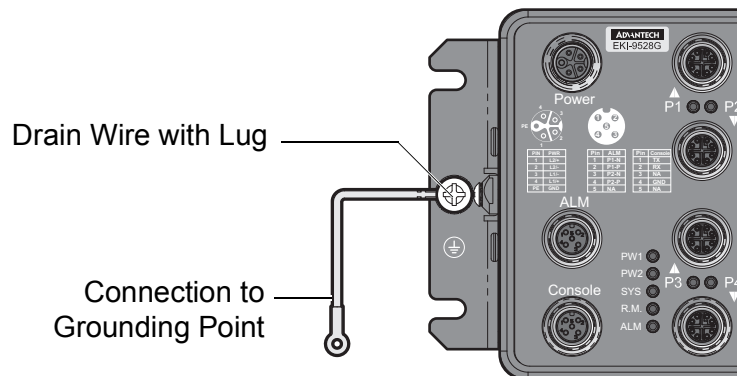
Figure 2.6 Grounding Connection, Chassis Left Side View
