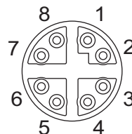
Figure 2.10 M12 X-Coded Connector Pin Assignment
