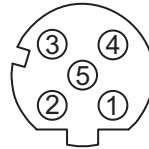
Figure 2.9 M12 D-Coded Connector Pin Assignment
