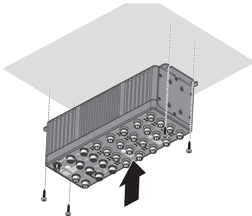
Figure 2.1 Installing a Switch on a Ceiling
