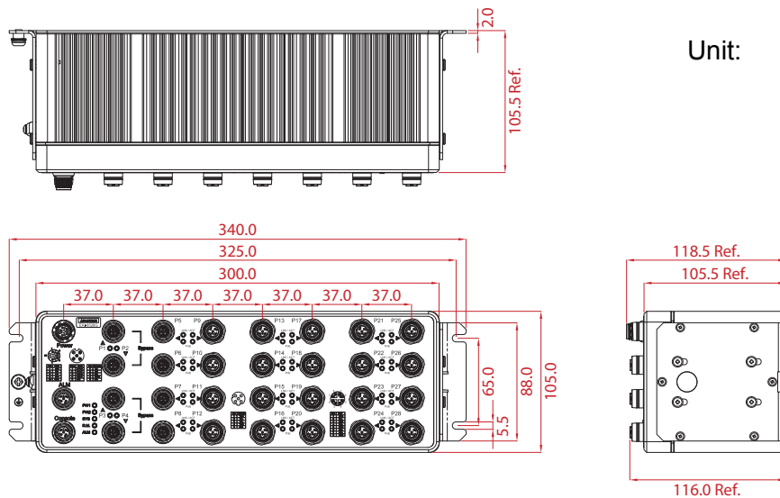
Figure 1.3 Dimensions
