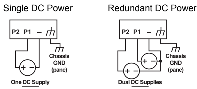
Figure 2.5 Power Wiring
